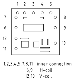
TERMINAL BOARD
